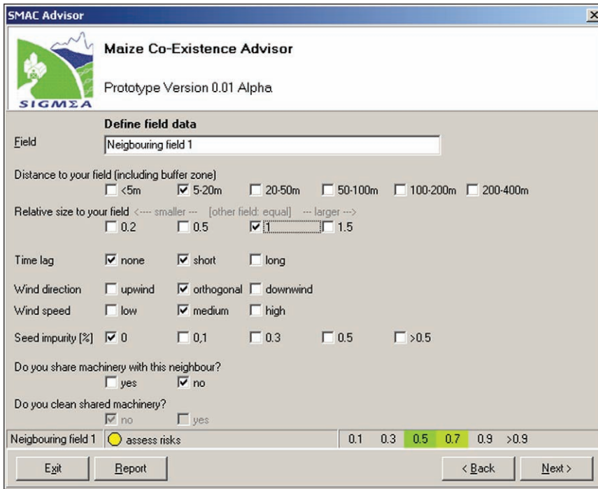
Figure 4. Description of SMAC Advisor user interface.
