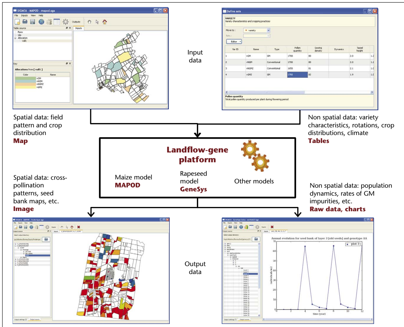
Figure 2. General Structure of LandFlow-Gene uses spatial information on landscape patterns and crop allocation as well as information on crop management, climate and varieties to estimate the proportion of GM material in non-GM crop production. Outputs can be obtained at the field level (average mean of adventitious presence) or for small units (intra-field adventitious presence).
